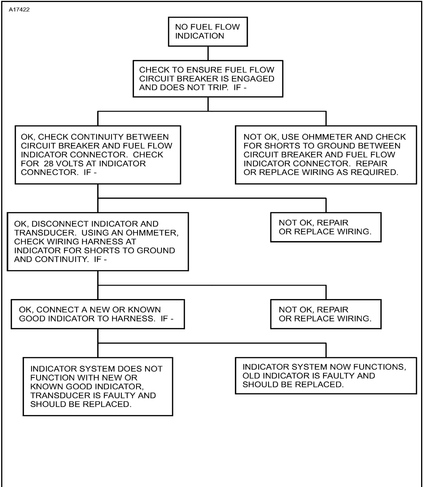
Figure 101 : Sheet 1 : Fuel Flow Indicator Troubleshooting Chart
